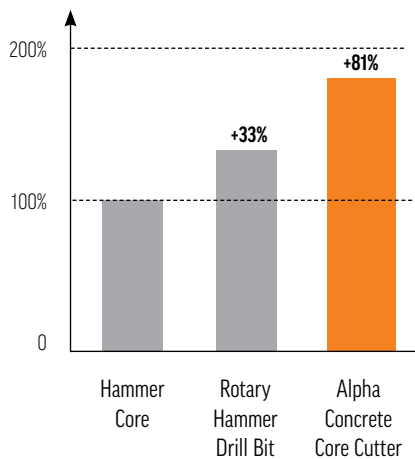
Significantly improved performance when drilling steel reinforcement
